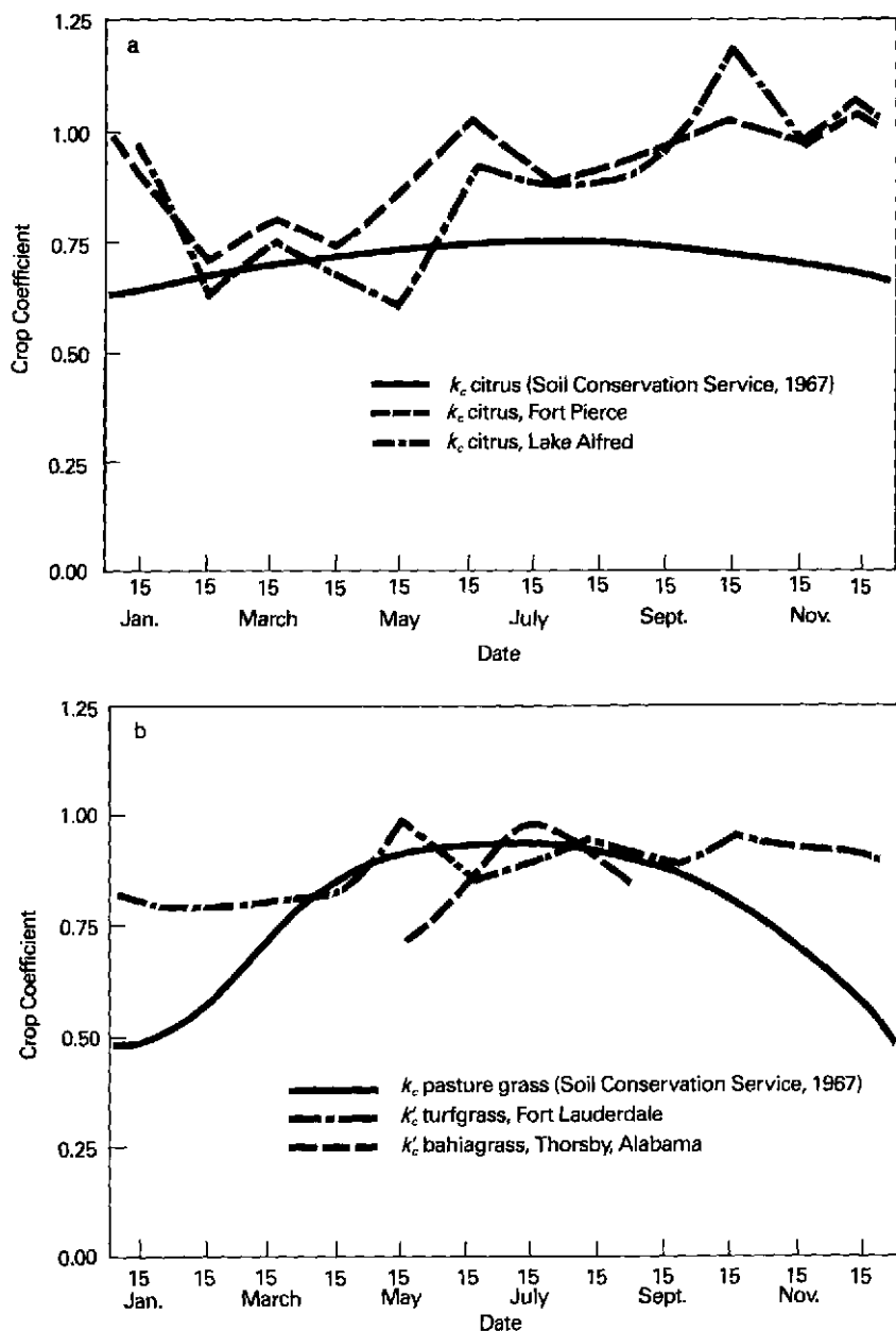
Fig. 10. Crop coefficients for (a) citrus and (b) pasture and turfgrass reported by USDA-SCS (1967) for a modified Blaney-Criddle approach applied to estimate ET_p ( k_c ) and those calculated from data presented in this report, using Penman estimates of ET_p ( k_c' ).
