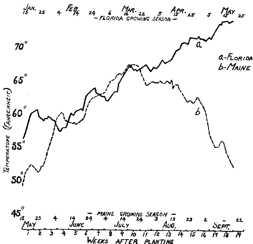
Fig. 2.—Daily average mean temperatures during the periods 1917-1926 and 1916-1926* for the potato-growing seasons at Federal Point, Florida, and Aroostook Farm, Presque Isle, Maine, respectively.
