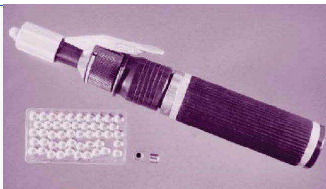
Above: Penetrating captive bolt and charges
