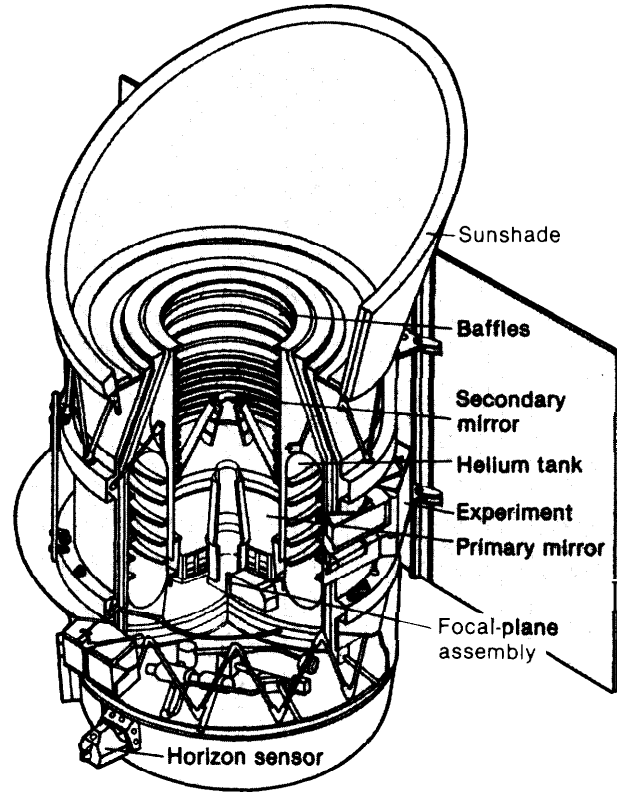
Figure 4-6.—Deep Space Surveillance Systems
