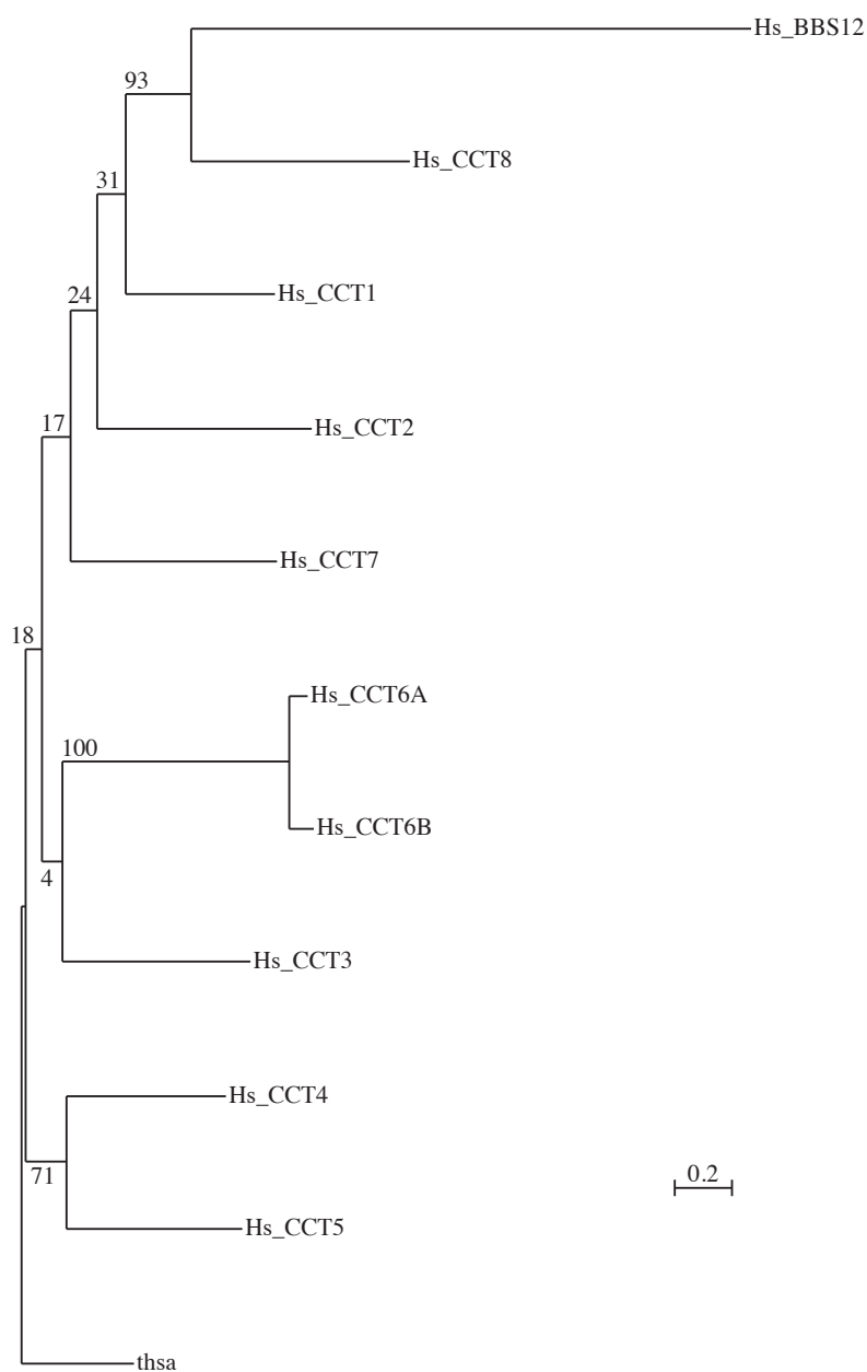
Figure S4. ML tree of CCT proteins with BBS12, excluding other BBS proteins and CCT8L proteins. "thsa" is the Thermoplasma acidophilum alpha subunit of the thermosome. The scale bar represents the indicated number of substitutions per position for a unit branch length.
