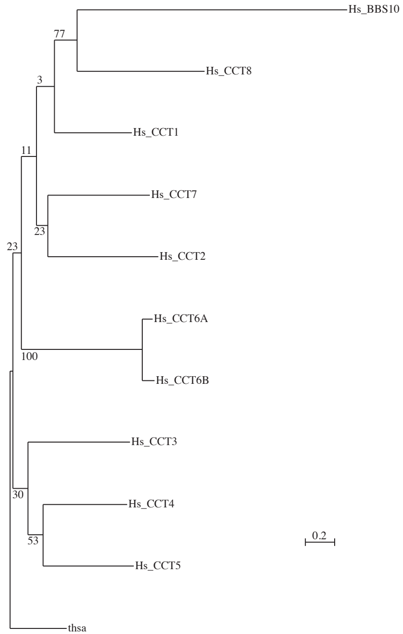
Figure S3. ML tree of human CCT proteins with BBS10, excluding other BBS proteins and CCT8L proteins. "thsa" represents the Thermoplasma acidophilum alpha subunit of the thermosome. The scale bar represents the indicated number of substitutions per position for a unit branch length.
