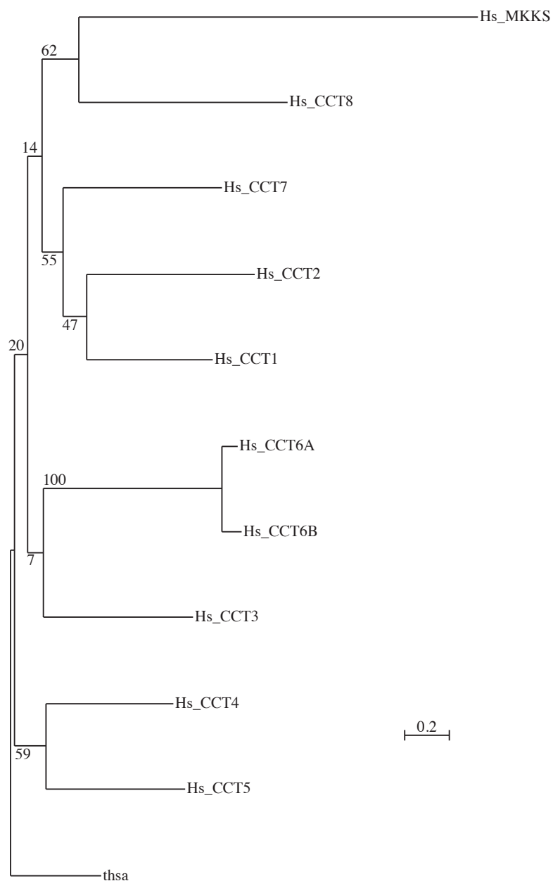
Figure S2. ML tree of human CCT proteins with MKKS (BBS6), excluding other BBS proteins and CCT8L proteins. "thsa" represents the Thermoplasma acidophilum alpha subunit of the thermosome. The scale bar represents the indicated number of substitutions per position for a unit branch length.
