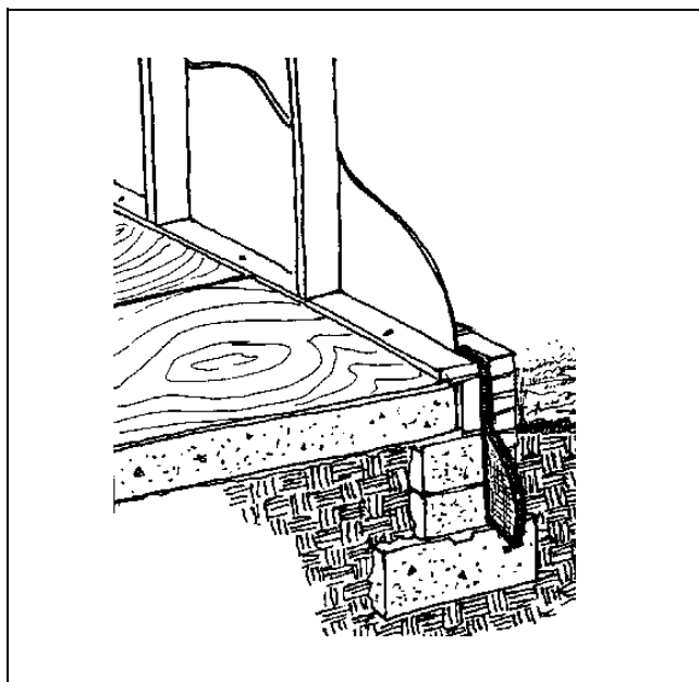
Figure 20. North Florida on-grade slab houses should have perimeter insulation.
