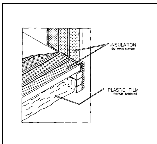
Figure 14. Condensation temperature occurring at vapor barrier (stud wall).
