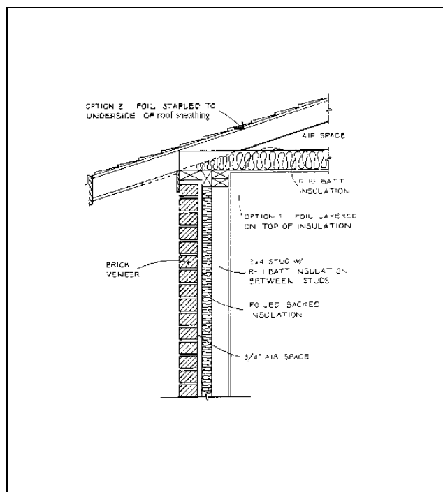
Figure 19. Radiant barrier applications.
