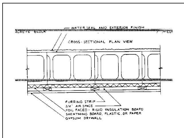
Figure 17. Block wall insulation on inside.
