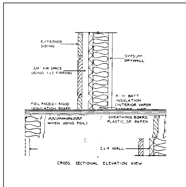
Figure 16. Frame wall insulation.
