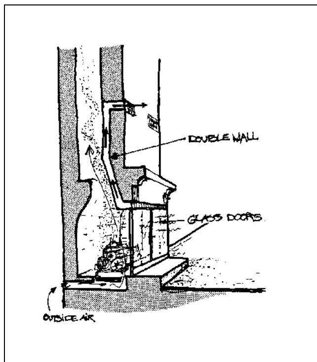
Figure 28. Energy saving fireplaces provide outside air for combustion.
