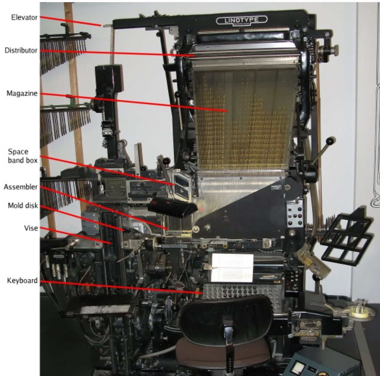
Figure 6.22: A Linotype type-casting system.
