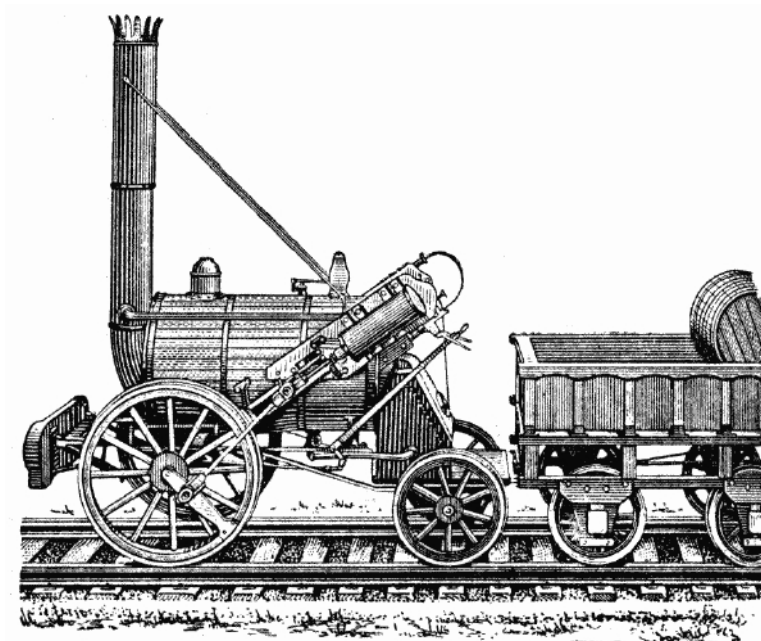
Figure 6.17: Drawing of the locomotive Rocket.
