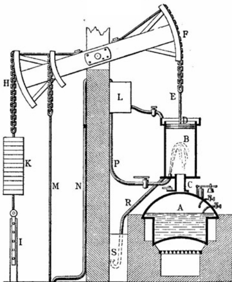
Figure 6.12: A drawing of the Newcomen steam engine. The letter “D” marks the piston that moves up and down in the cylinder.
