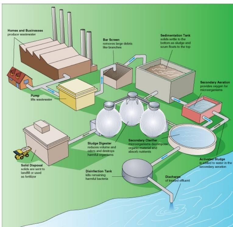
Figure 3.10: Steps in a typical wastewater treatment process.
