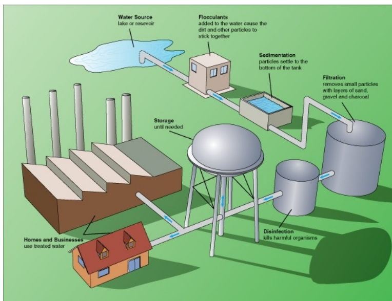
Figure 3.8: Illustration of a typical drinking water treatment process.
