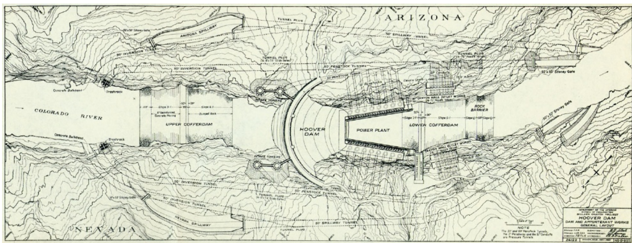
Figure 6.37: A contour map of Hoover Dam and the surrounding canyon.
