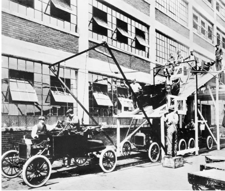
Figure 6.24: Part of a Ford assembly line.
